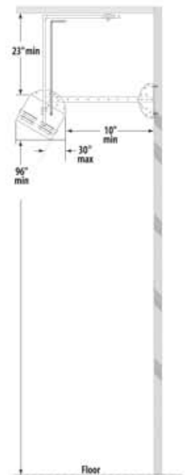
30 ° installation to combustible surface (side view)
