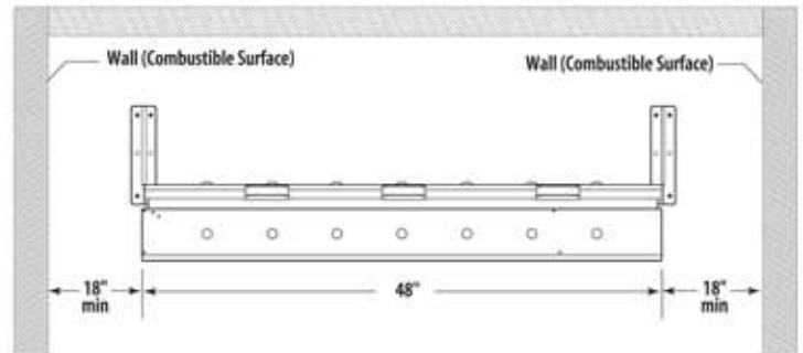
0 ° installation to combustible surface (side view)
